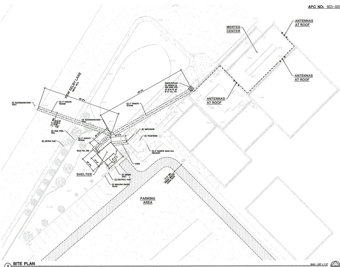
1 SITE PLAN
